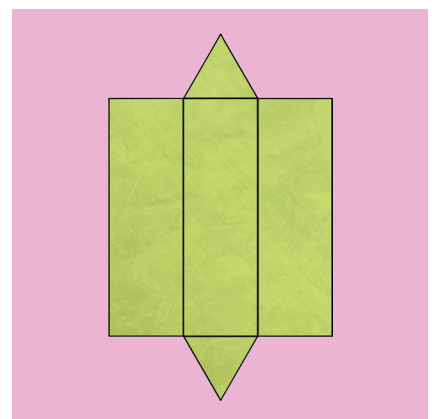
triangular prism
