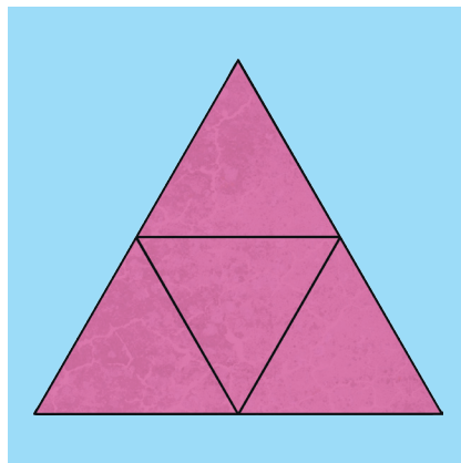
tetrahedron
