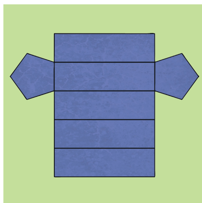
pentagonal prism
