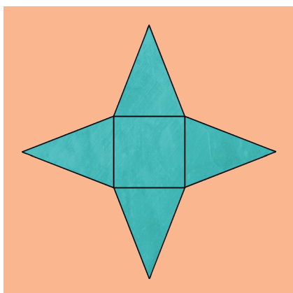
square-based pyramid
