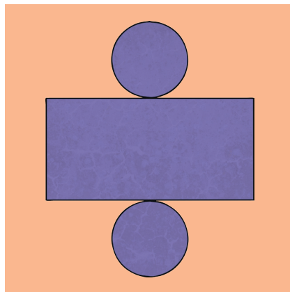
cylinder
