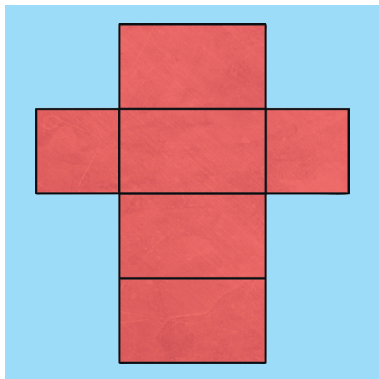
cuboid
